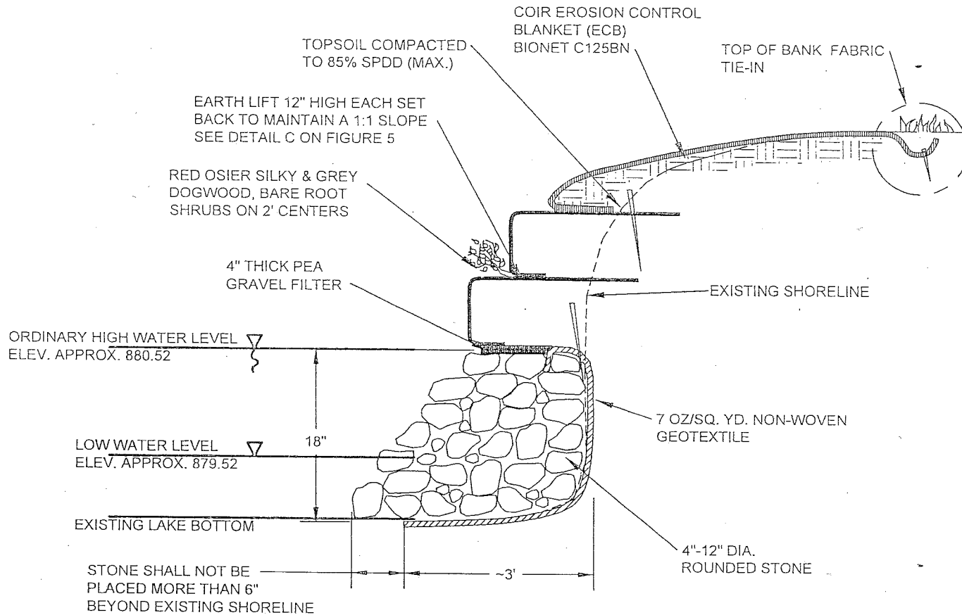
A 3 TYPICAL FABRIC ENCAPSULATED SOIL LIFT/ROCK TOE - DETAIL NOT TO SCALE
