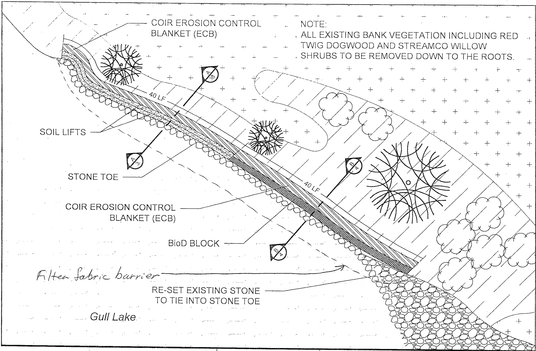
Figure 2 : PROPOSED SITE PLAN KBS SHORELINE MANAGEMENT DEMONSTRATION AREA
